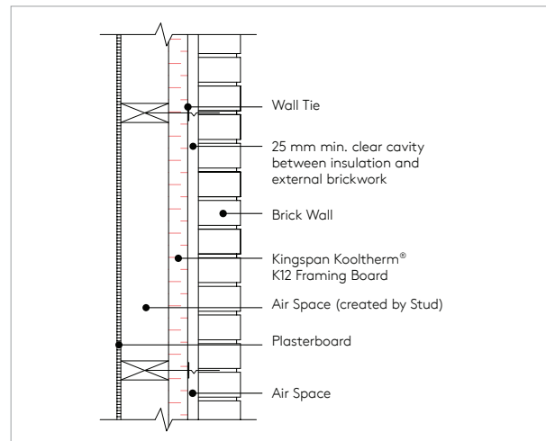
Figure 7. Side elevation – Brick Veneer wall with Kingspan Kooltherm® K12 Framing Board.
