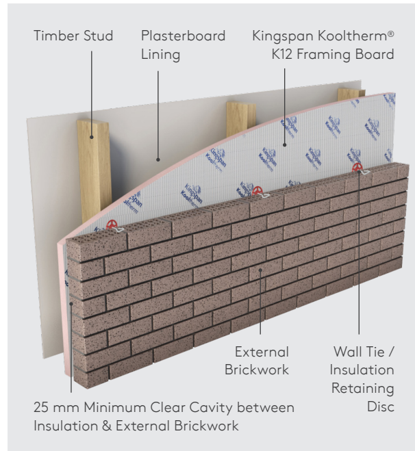
Figure 2. Brick Veneer Installation with Kooltherm® K12 Framing Board installed on External Side of Timber Framing.
