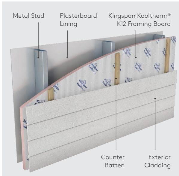
Figure 3. Steel Framed Wall Installation.
