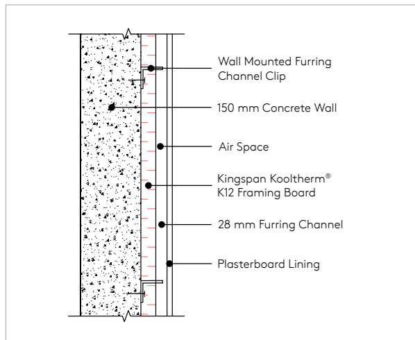
Figure 6. Side elevation of Kingspan Kooltherm® K12 Framing Board clip-and-channel system.
