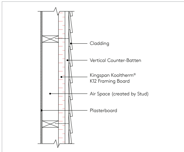
Figure 8. Side elevation – Stud wall with Kingspan Kooltherm® K12 Framing Board and vertical counter-battens using an internal plasterboard lining.
