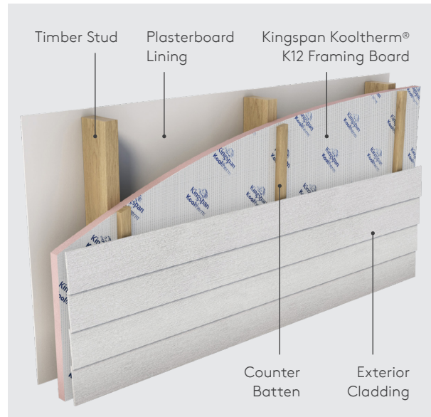
Figure 4. Timber Framed Wall Installation.
