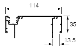
Offset Glazing Frame CI-3233 (CI-7632)
