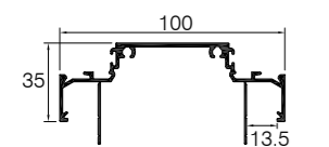
Double Glazing Sill CI-2252 (CI-6445)
