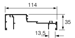
Window Sill CI-3250 (CI-7605)
