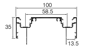
Double Glazing Frame CI-2232 (CI-6442)
