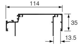
Offset Glazing Sill CI-3253 (CI-7635)
