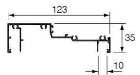
Window Sill CI-4950 (CI-9105)
