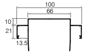
Ceiling Channel (10mm shadowline) CI-2211 (CI-6401)
