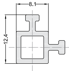
Corner connection M for 4 mm
