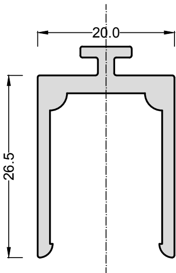
Basic profile M
