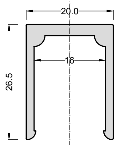
Cover profile
