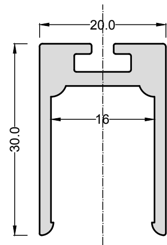
Basic profile F
