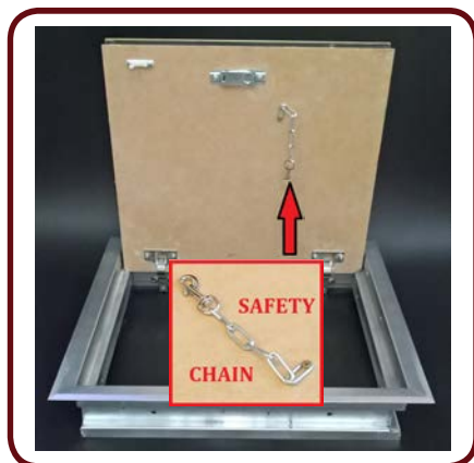
FEATHERED FLANGE
