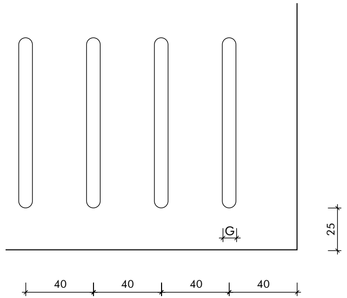
02 SLOTTING DETAIL Scale - NTS
