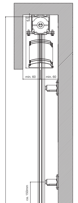
CHANNEL GUIDE
