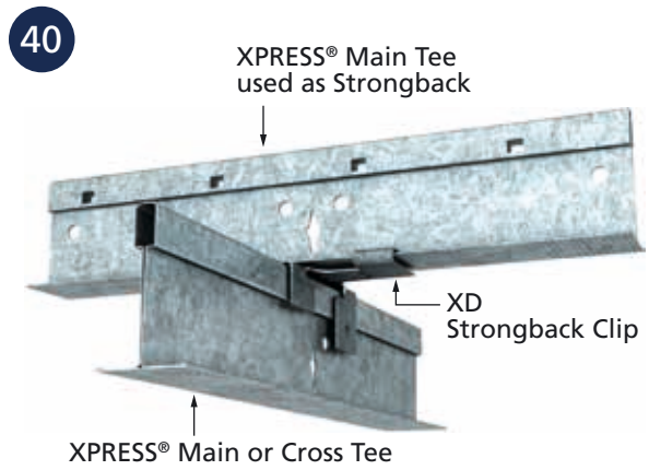
■ XD19 STRONGBACK CLIP INSTALLED
