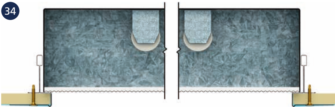
■ TYPICAL DETAIL: LAY-IN LIGHT FIXTURE
