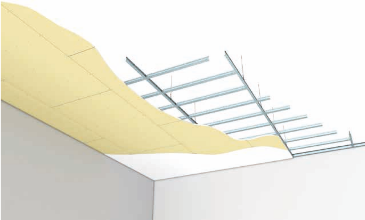
■ TYPICAL RONDO XPRESS® DRYWALL GRID CEILING WITH LIGHT FIXTURE AND ACCESS PANEL
