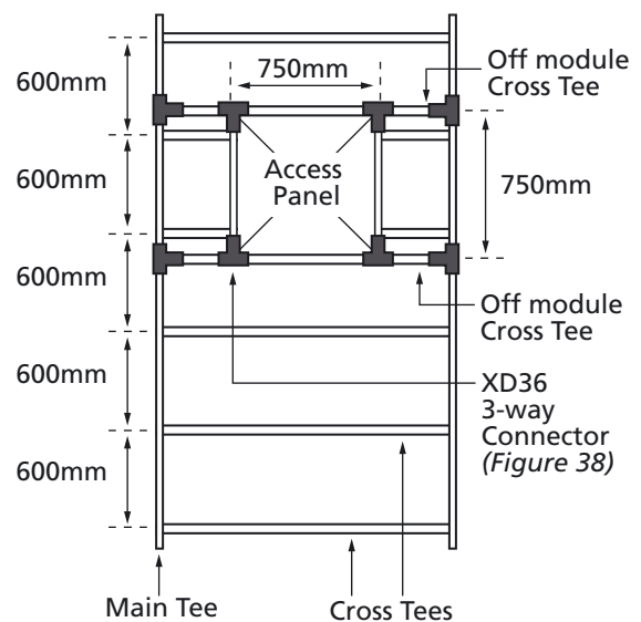
■ PANTHER® ACCESS PANEL OFF MODULE LAYOUT
