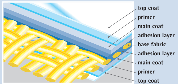
Schematic sectional drawing of VALMEX ® FR MEHATOP F
