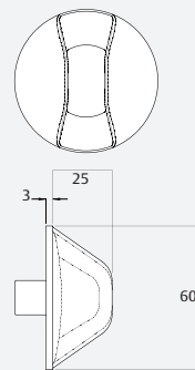
Standard Knob 21
