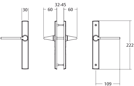
Aria® #27
