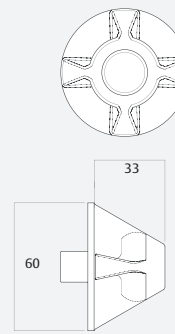
Webbed Knob 22
