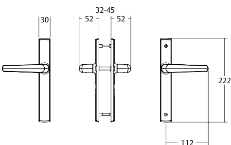
Aria® #27
