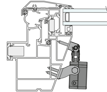
Roof window, outward opening
