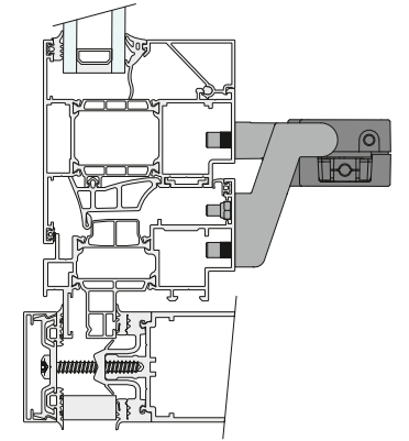
Façade windows, outward opening
