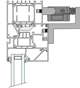
Façade windows, inward opening
