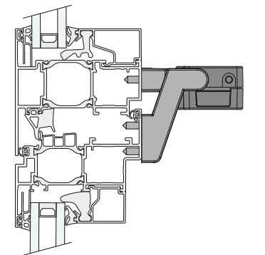
Universal bracket sets, outward opening
