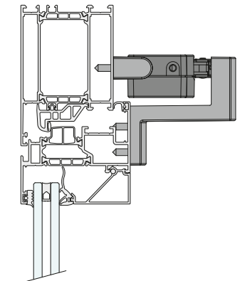
Universal bracket sets, inward opening
