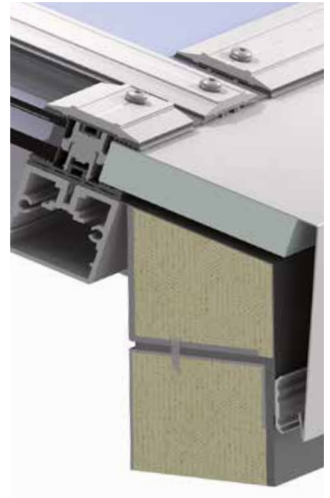
INSTALLED ON STEEL SHEET FRAME
