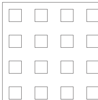
pattern 12/25Q dimensions: 1200 x 2000 x 12.5mm perforated area: 23.0% mass per unit area: 7.7kg/m 2
