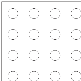
pattern 12/25R dimensions: 1200 x 2000 x 12.5mm perforated area: 18.1% mass per unit area: 8.2kg/m 2
