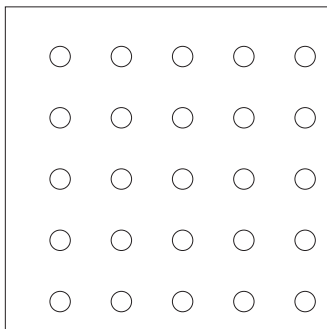
pattern 6/18R dimensions: 1188 x 1998 x 12.5mm perforated area: 8.7% mass per unit area: 9.1kg/m 2
