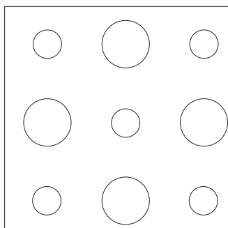
pattern 12/20/66R dimensions: 1188 x 1998 x 12.5mm perforated area: 19.6% mass per unit area: 8.0 kg/m 2
