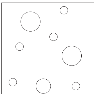
pattern 8/15/20R dimensions: 1200 x 2000 x 12.5mm perforated area: 9.5% mass per unit area: 9.1kg/m 2
