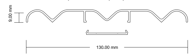
Triple Track & Snap Strip Dimensions
