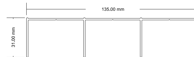
Headguide Channel Dimensions
