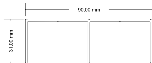
Headguide Channel Dimension
