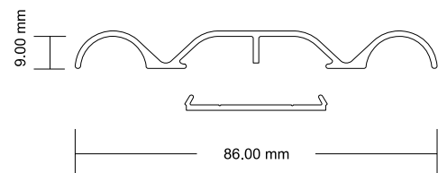
Double Track & Snap Strip Dimensions
