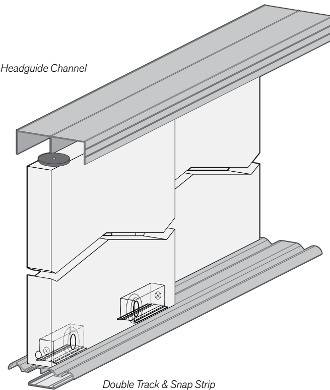
Double Track & Snap Strip
