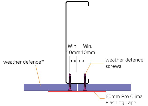
FIGURE 11 Typical joint detail
