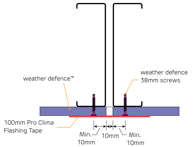
FIGURE 13 Vertical control joint detail
