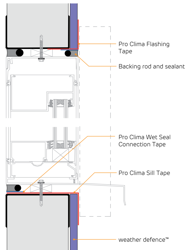
FIGURE 18 Window head and sill detail
