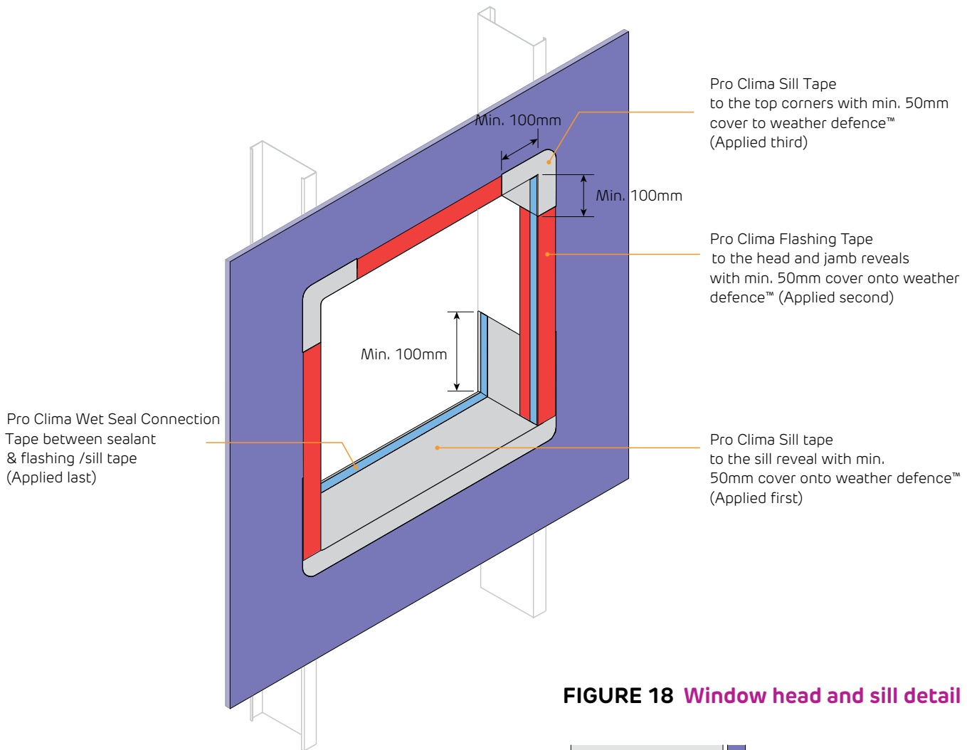
FIGURE 16 Isometric view of window/meter box opening - tape application
