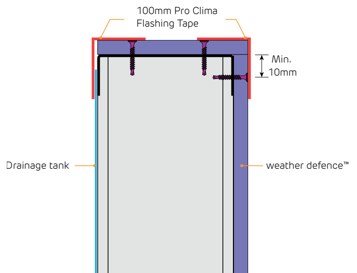
FIGURE 22 Parapet detail
