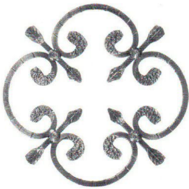
Art. 1-01 □ 8x8 mm ∅ 250 mm 0.780 kg
