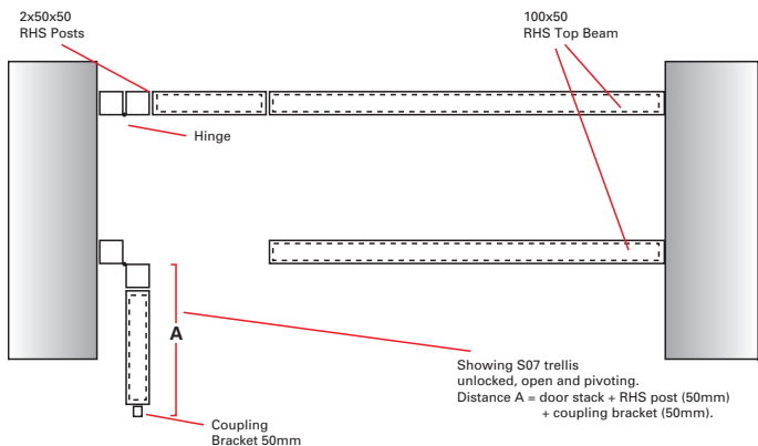
Plan View
