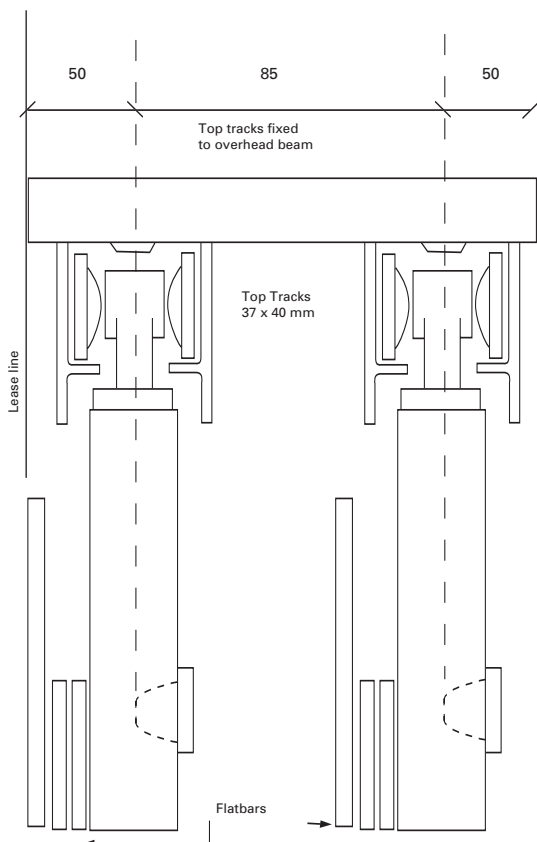
Sectional View
