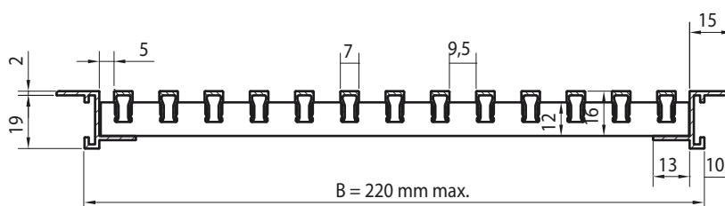
394/2: linear bar grille with flanged 'Z' frame
