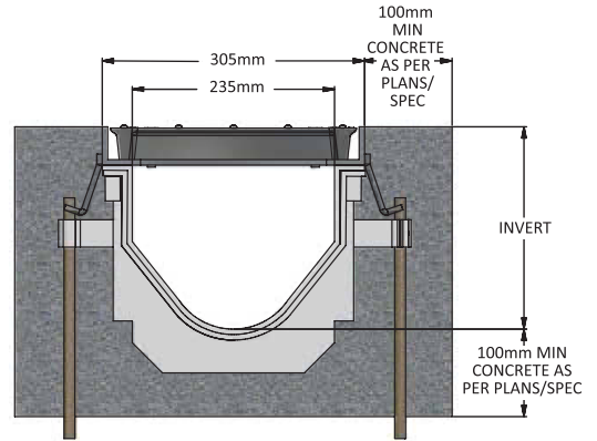
Bottom Outlet (U6, U8, 150mm, 225mm)
