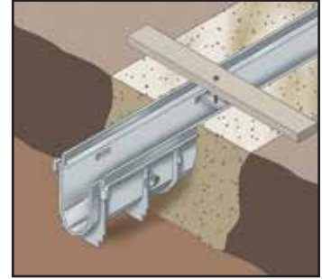
Suspended Installation Z886 Perma-Trench Illustrated
