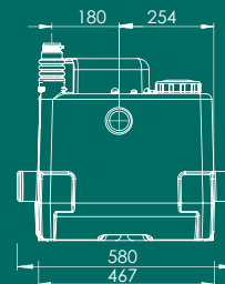
External mounted control box
