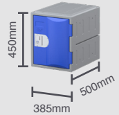
QUARTER HEIGHT
