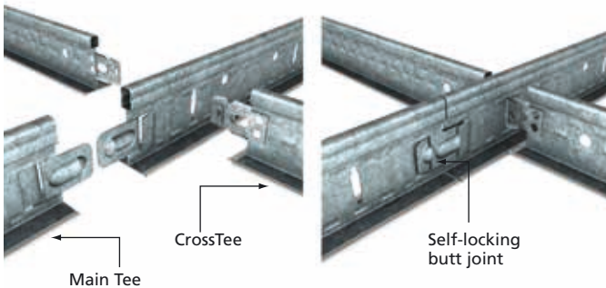
■ FIGURE 5: MAIN AND CROSS TEE JOINTING CROSS
