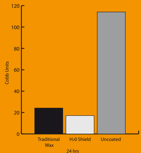
Cobb Test - Measure of Water Up-take
