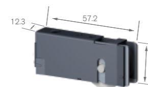
Sliding Window Rollers DR142 Window Roller (7.5 kg) DR142 SS Window Roller (15 kg)
