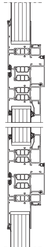
Systems cross section Series 85
