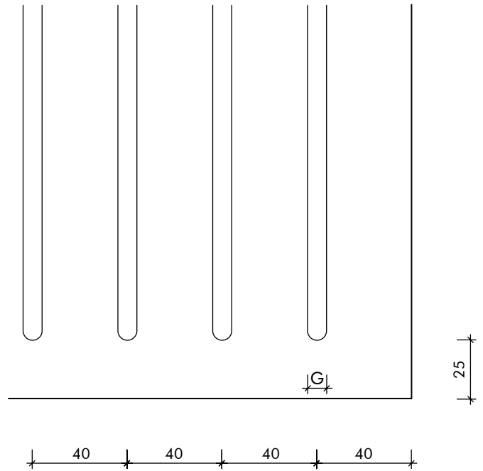
02 SLOTTING DETAIL Scale - NTS
