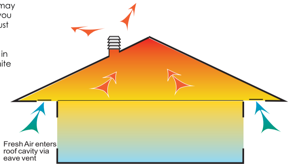
Venting attic void
