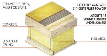
STANDARD CONFIGURATION FLOOR/CEILING ASSEMBLY (WITH SUSPENDED CEILING/INSULATION)
