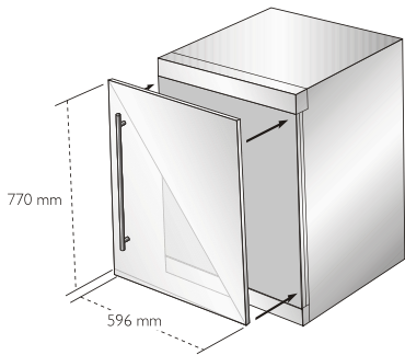
Door Dimension for Fully Integrated
