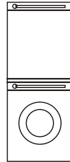
Single pull-out drawer located between washer and dryer 1730 height 600mm width 600mm depth
