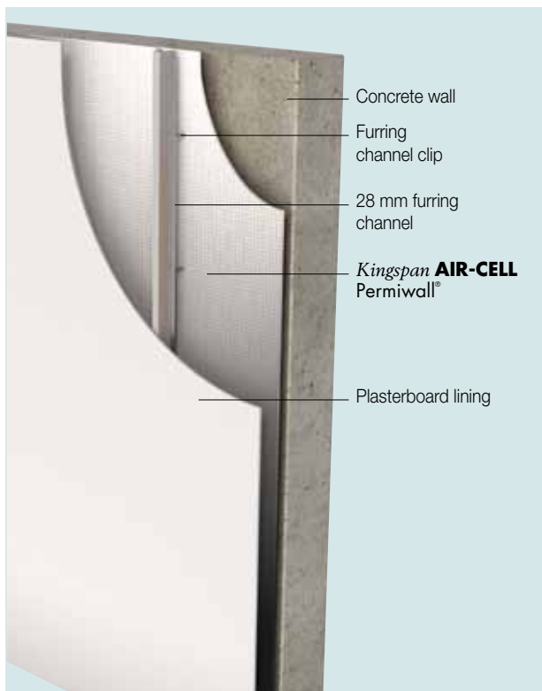
Figure 1 Kingspan AIR-CELL Permiwall clip-and-channel system
