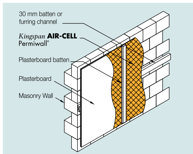
Figure 3 Kingspan AIR-CELL Permiwall counter-batten system
