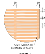
DETAIL A 5mm RADIUS TO CORNERS OF SLOTS
