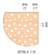
DETAIL A 1:10
