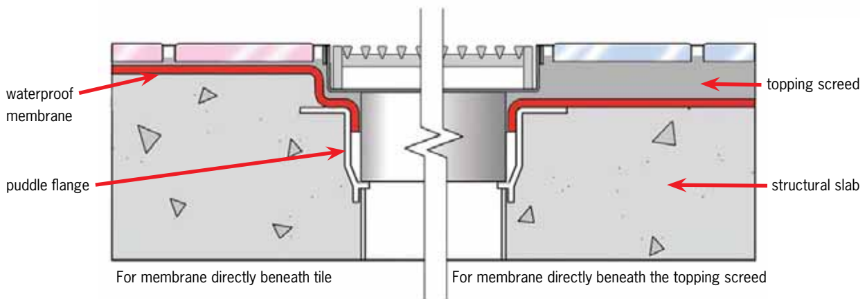
Trough Detail
