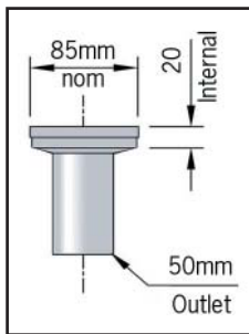
Trough Detail
