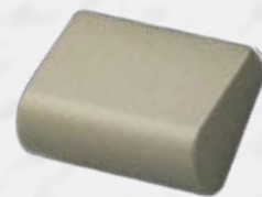
Art: 114030 Size Length Height Centres Projection 26mm 10mm 16mm 20mm Finish | Nickel
