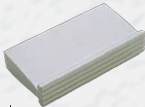
Art: 49163 Size Length Height Centres Projection 45mm 9mm 32mm 24mm Finish | SAA
