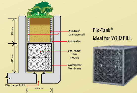
Flo-Cell® 20mm
