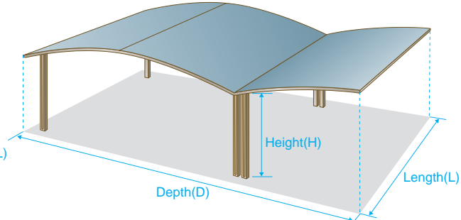
M+Y-Connection
