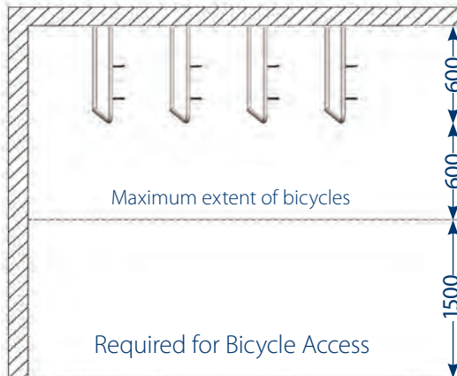
CVR3 (Plan view)
